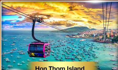
Hon Thom Island
